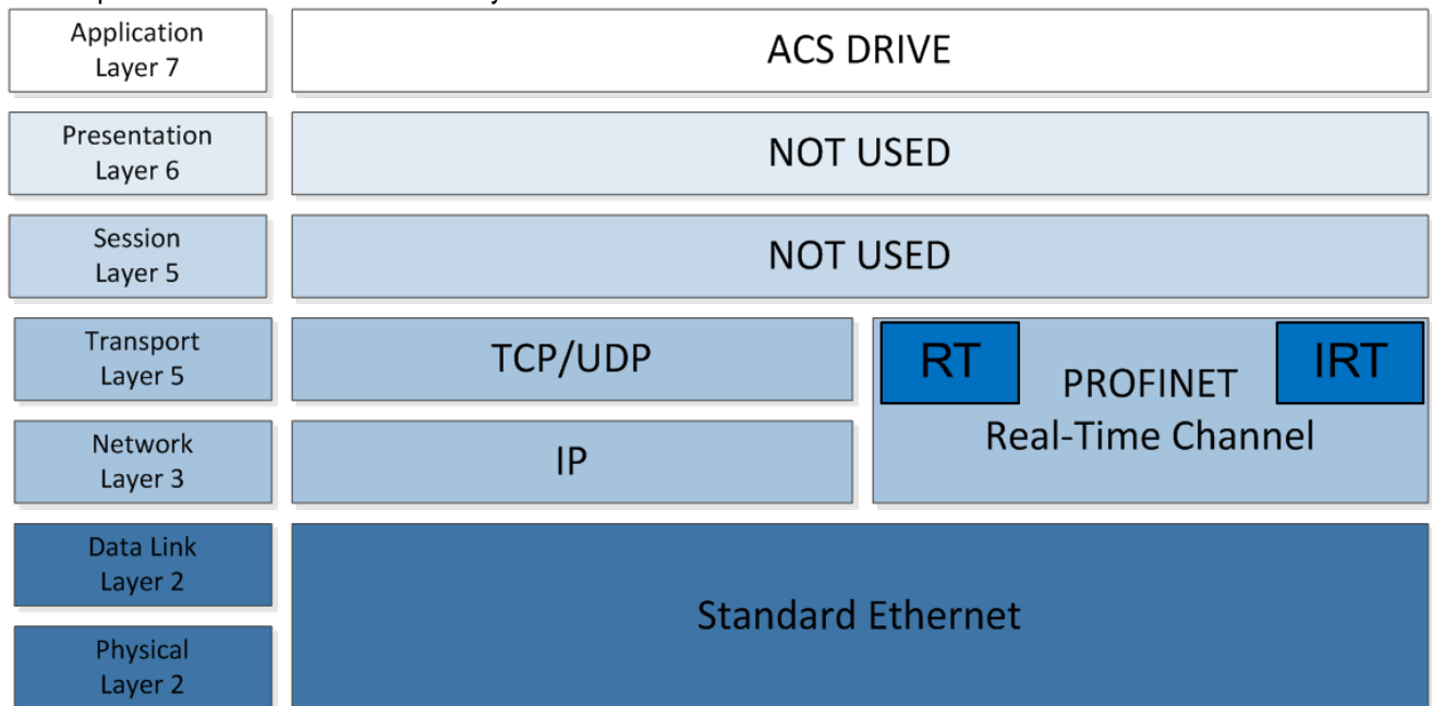
Figure 1: PROFINET OSI Network Layer Model
