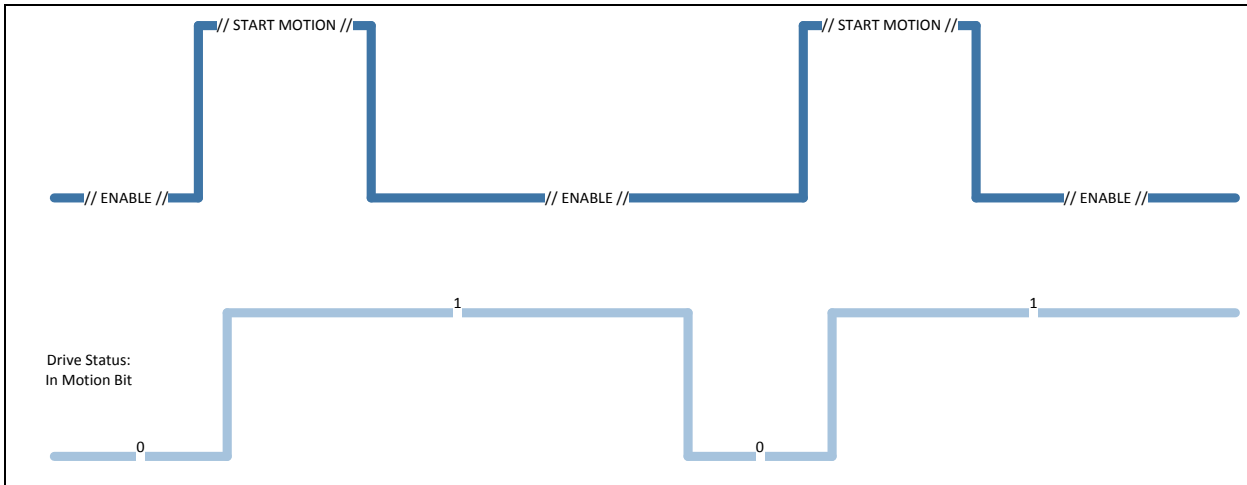
Figure 2 - Edge Triggered Commands
