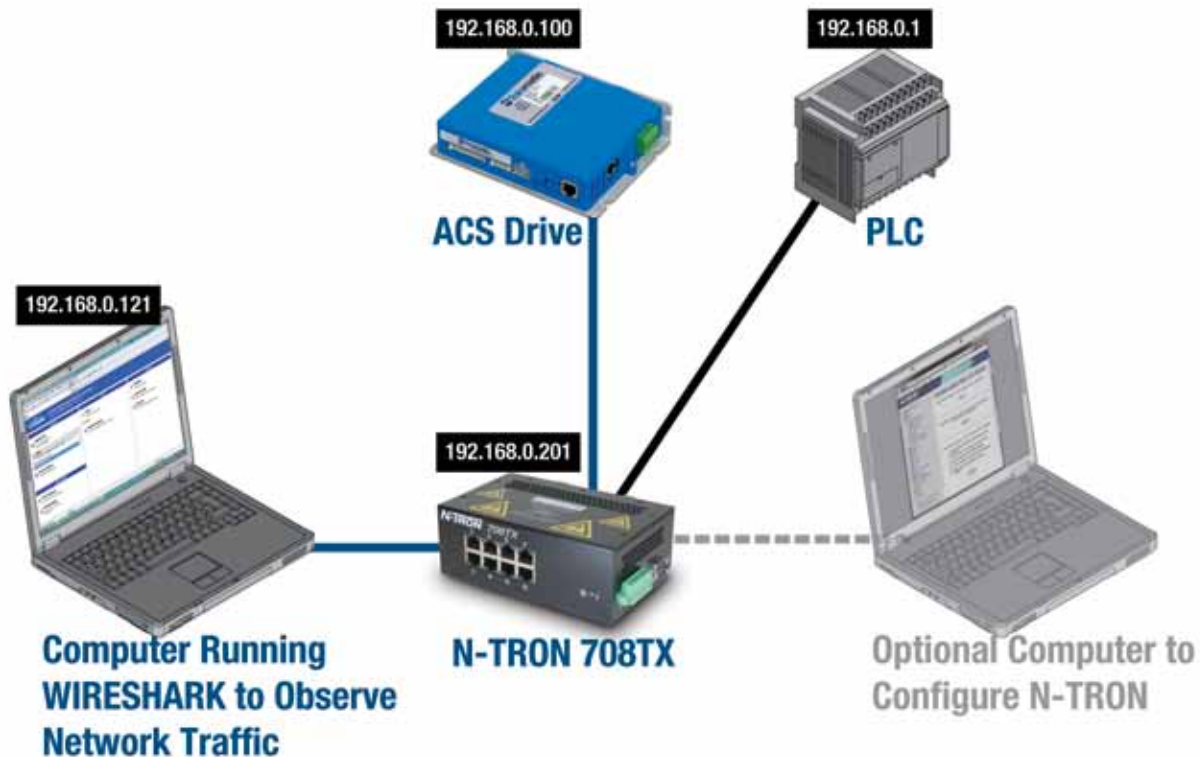
Figure 1: System Overview, make connections as shown in diagram above
