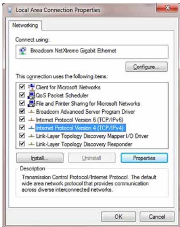
Figure 4: Entering Properties of TCP/IPv4
