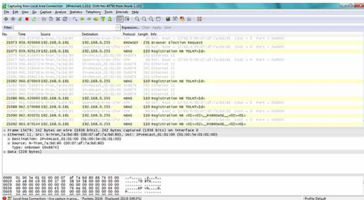
Figure 12: WIRESHARK Network Traffic
