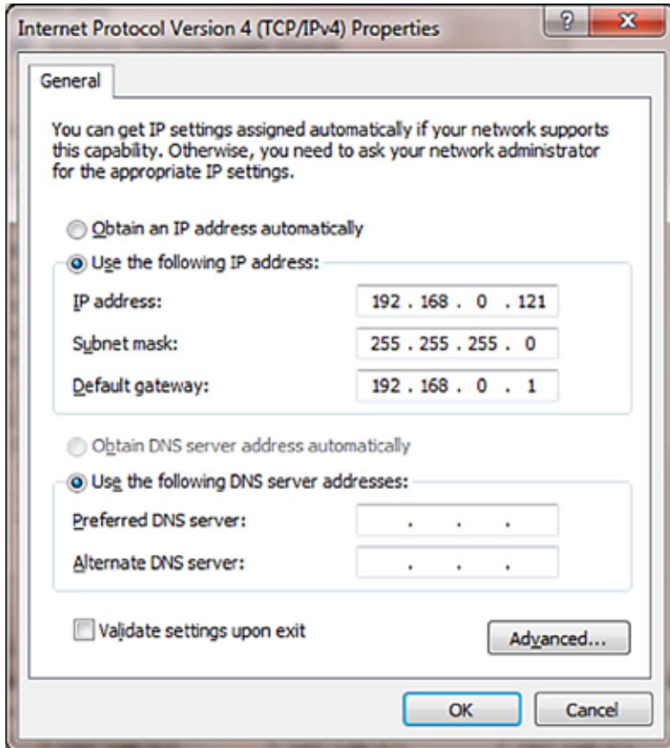
Figure 5: Setting the PC Network IP address
