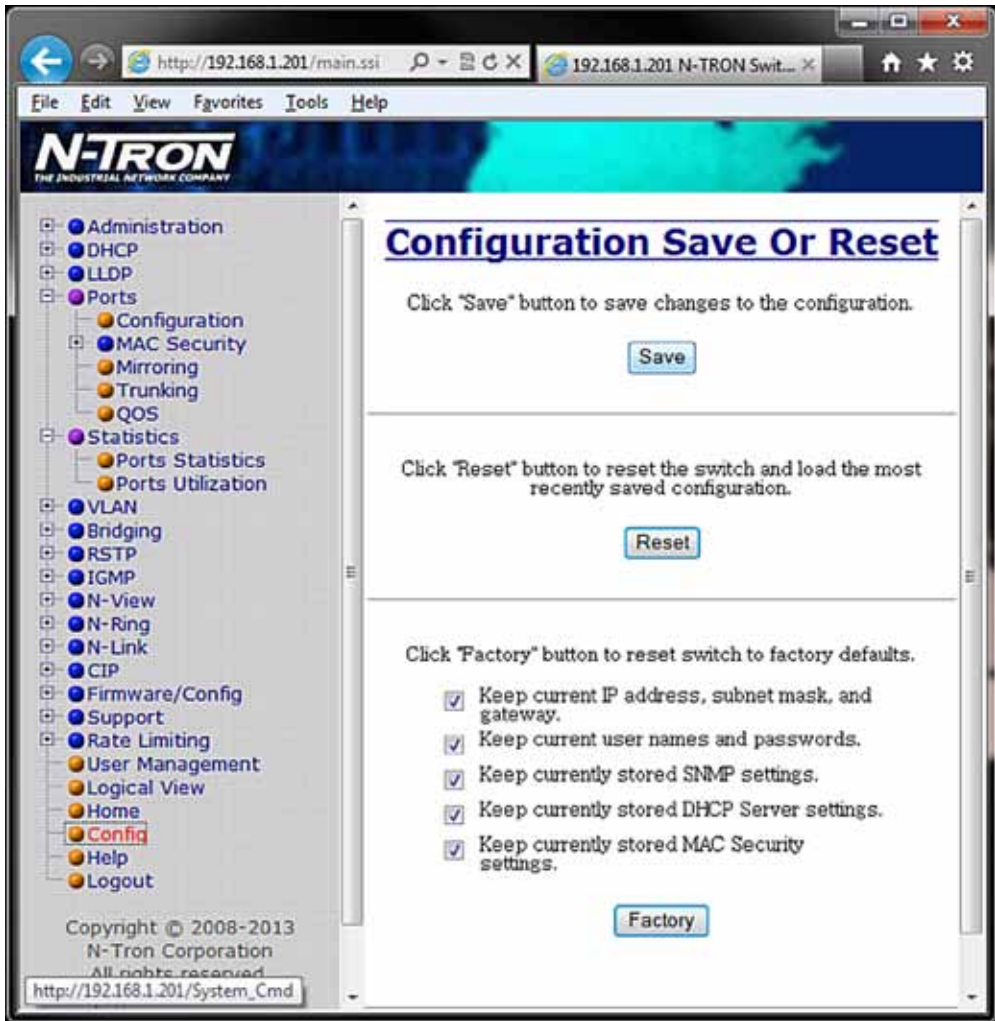
Figure 10: Configuration Save Screen
