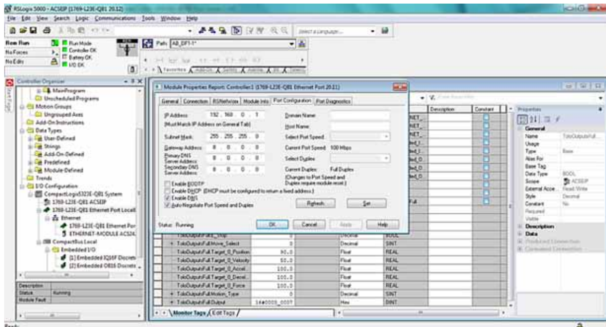
Figure 14: IP address configuration in RSLogix5000
